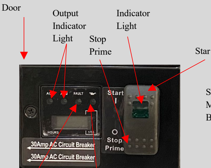
Start/Stop Switch inside Generator Service Access Door
