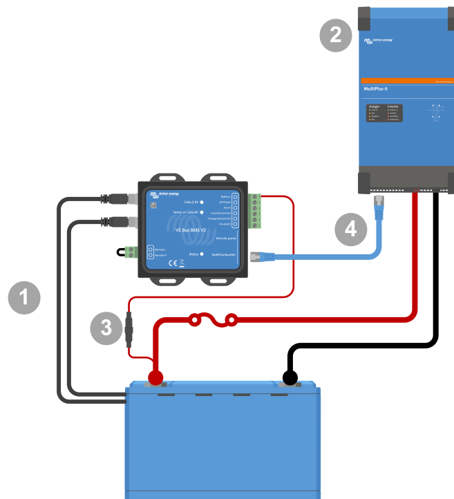
Basic BMS connections
