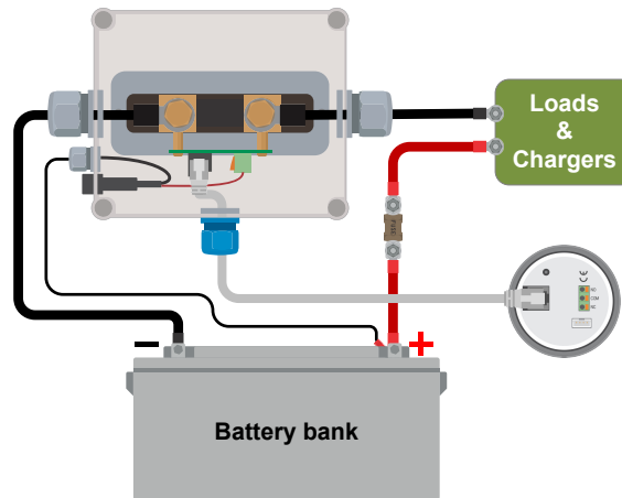
Basic battery monitor installation.
