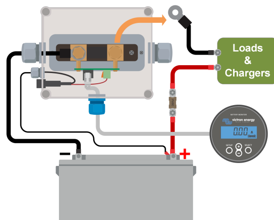
Performing a zero current calibration.
